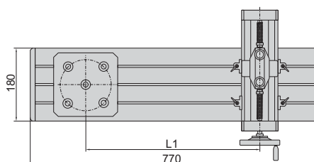
adaptor (optional, for digital torque tester IST-TT5 , IST-TT30 , IST-TT50 , IST-TT220 )
