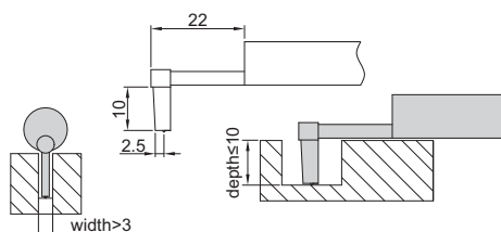
deep groove probe (optional), code ISR-C002-DGP
