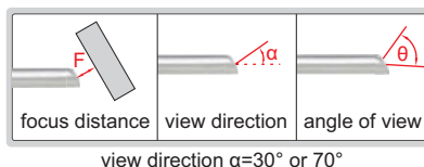
view direction α=30° or 70°
