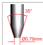
blunt taper indenter
