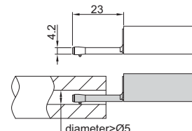
small hole probe (optional), code ISR-C002-PROBE
